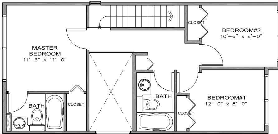
2nd Floor
